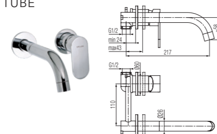
Concealed wall-mounted basin mixer
