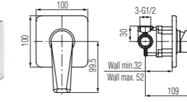
Concealed shower mixer
