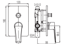
Concealed bathtub and shower mixer tap
