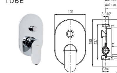
Concealed bathtub and shower mixer tap
