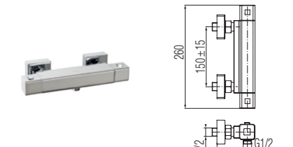
Thermostatic mixer for shower
