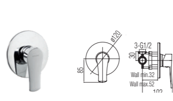
Concealed shower mixer
