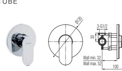
Concealed shower mixer
