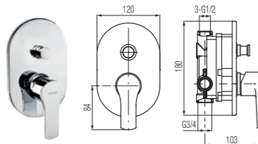
Concealed bathtub and shower mixer tap
