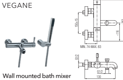
Wall mounted bath mixer
