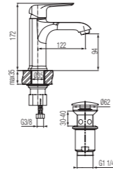
Washbasin high mixer
