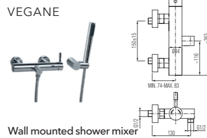
Wall mounted shower mixer
