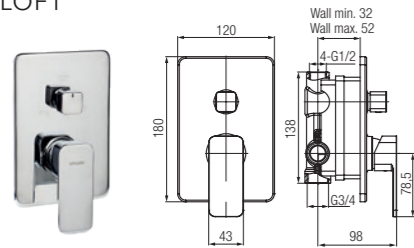
3-function concealed mixer
