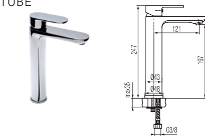
Washbasin high mixer
