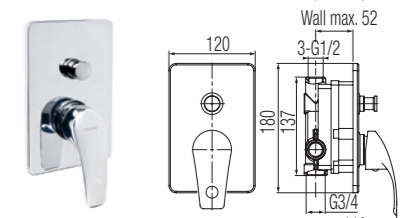
Concealed bathtub and shower mixer tap
