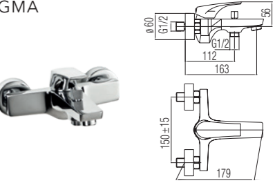
Wall mounted bath mixer
