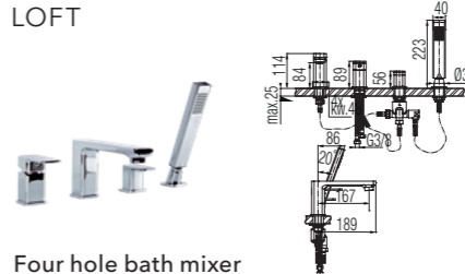
Four hole bath mixer
