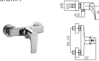
Wall mounted shower mixer
