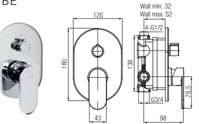
3-function concealed mixer
