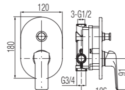
Concealed bathtub and shower mixer tap
