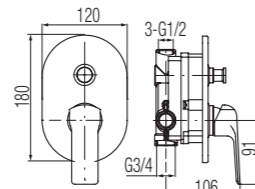
Concealed bathtub and shower mixer tap
