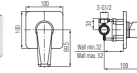
Concealed shower mixer
