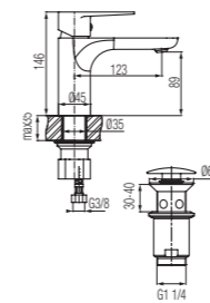
Washbasin high mixer
