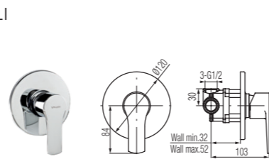
Concealed shower mixer
