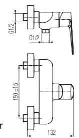
Wall mounted shower mixer
