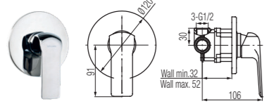
Concealed shower mixer
