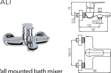
Wall mounted bath mixer
