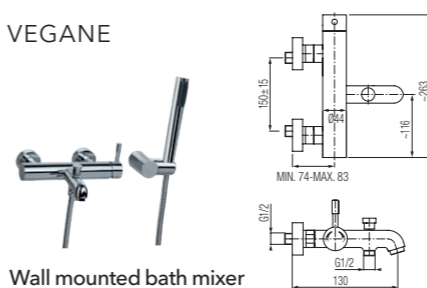
Wall mounted bath mixer
