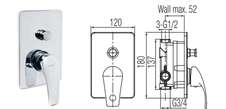
Concealed bathtub and shower mixer tap
