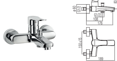
Wall mounted bath mixer
