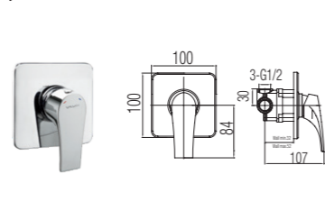
Concealed shower mixer
