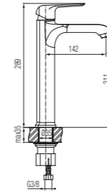
Washbasin high mixer
