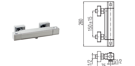
Thermostatic mixer for shower
