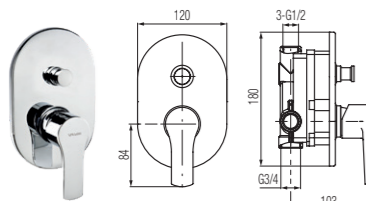
Concealed bathtub and shower mixer tap
