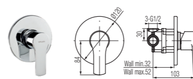
Concealed shower mixer
