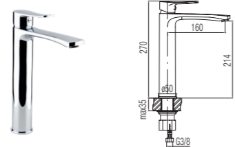
Washbasin high mixer
