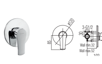
Concealed shower mixer
