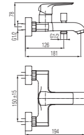
Wall mounted bath mixer
