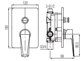
Concealed bathtub and shower mixer tap
