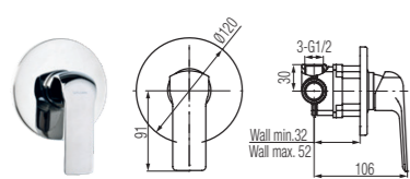
Concealed shower mixer
