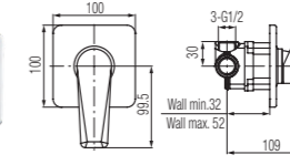
Concealed shower mixer
