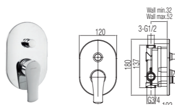
Concealed bathtub and shower mixer tap
