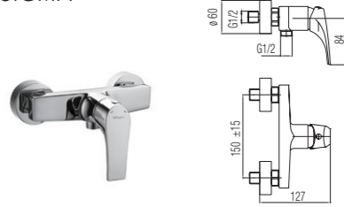
Wall mounted shower mixer
