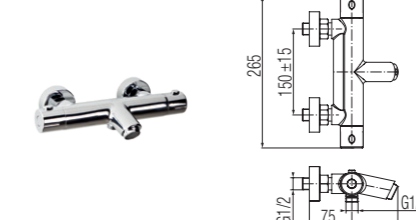
Thermostatic mixer for bathtub
