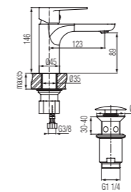
Washbasin high mixer
