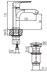
Washbasin high mixer
