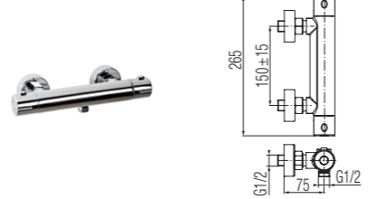
Thermostatic mixer for shower
