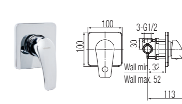
Concealed shower mixer
