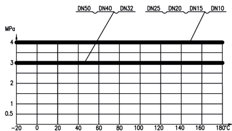
operating characteristic
