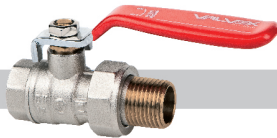
ONYX Full-port ball valve with nut on stem, with tail piece and steel lever
